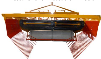
Pressure roller instead of wheels
